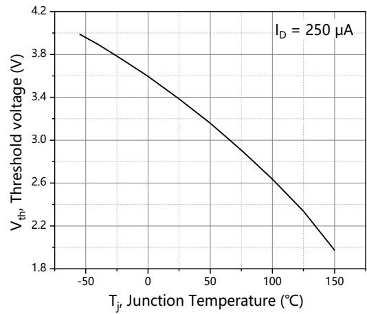
Figure 8. Threshold voltage
