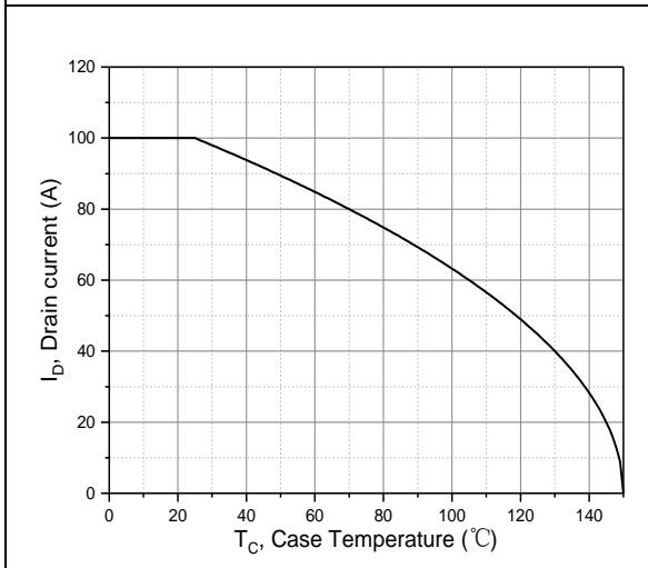
Figure 9. Drain current
