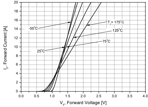
Figure 1. Forward Characteristics
