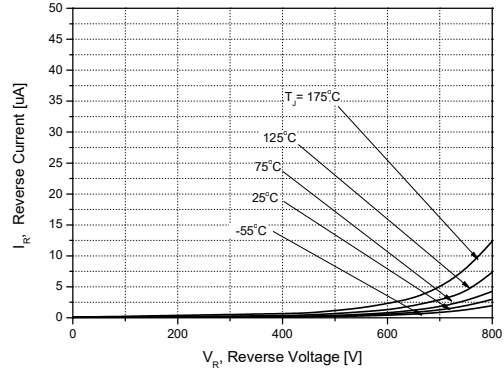
Figure 2. Reverse Characteristics
