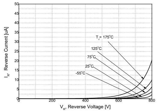
Figure 2. Reverse Characteristics
