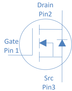
TO-247
